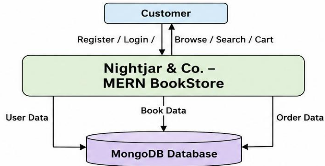
Figure 1: DFD Level 0 – Context Diagram
