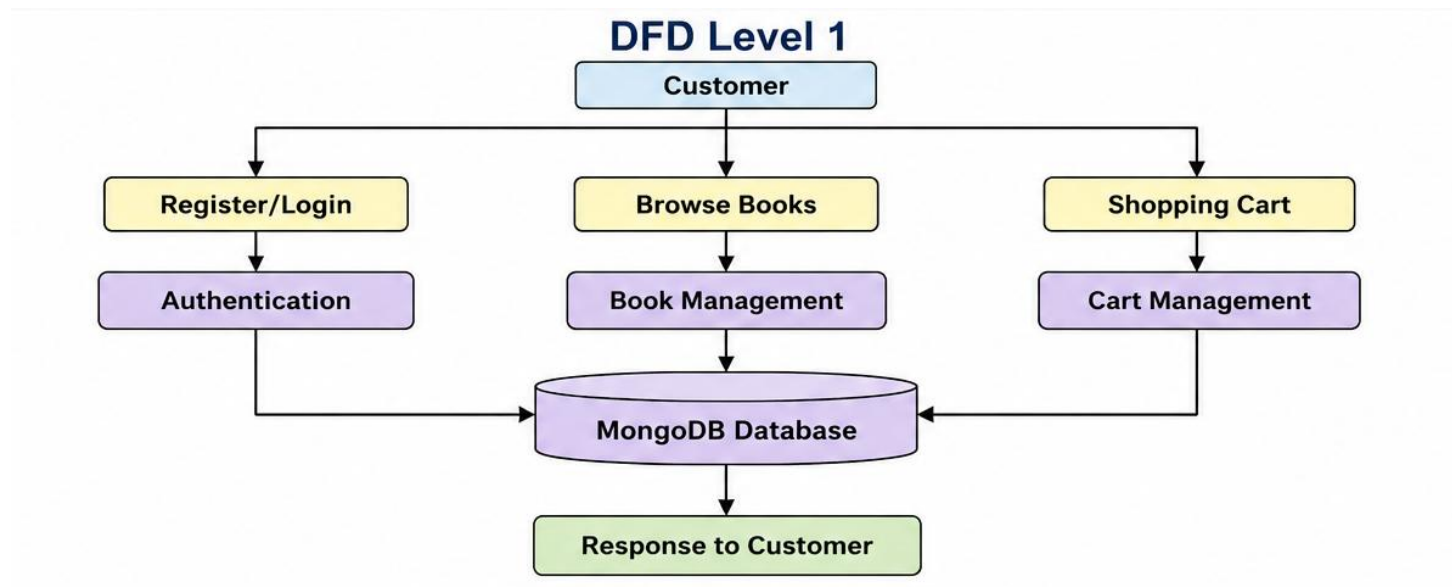
Figure 2: DFD Level 1 – System Processes
